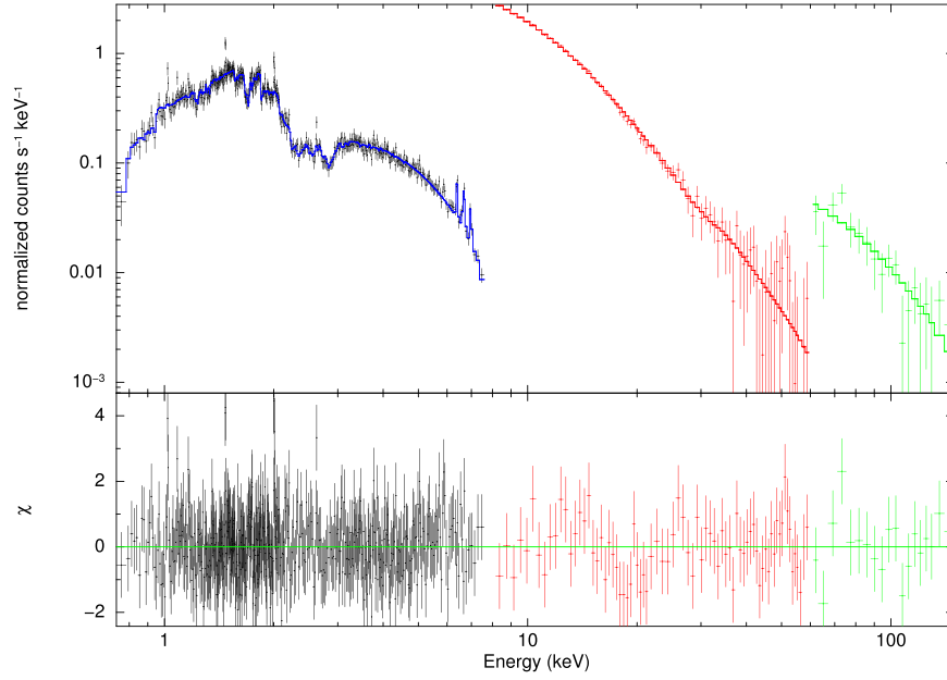
Figure 8. Spectral fit to the simultaneous Chandra/RXTE (ObsID 646/ObsID 50012-01-01-00) spectra of SS Cyg using the COMPTT+COMPTT+GAUSSIAN+GAUSSIAN+GAUSSIAN total model. The black, red, and green points correspond to 0.4–8.0 keV HETG/ACIS, 8.0–60 keV PCA, and 60–150 keV HEXTE data, respectively. The blue, red, and green lines correspond to the best spectral fit (see sixth column of Tables 7 and 8). The lower panel shows the residuals of the data vs. model.
